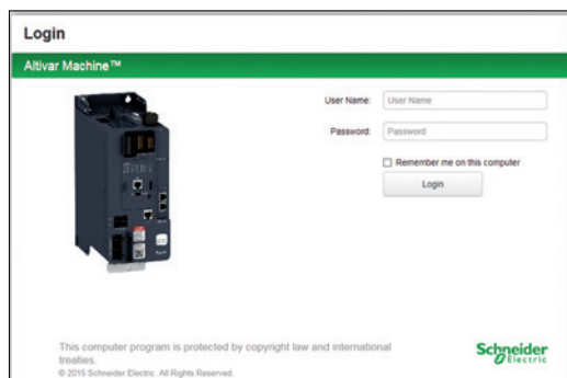
Login screen
