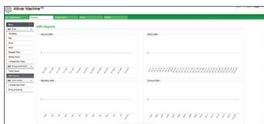
Energy dashboard
