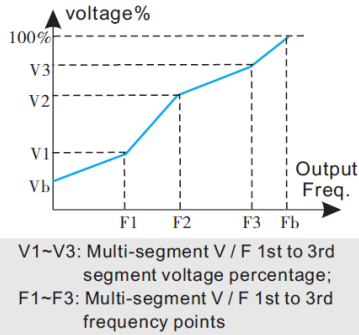
Fig 6-8 customized V/Fcurve
