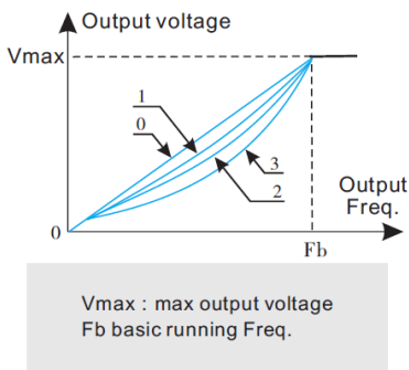
Fig 6-7 V/Curve
